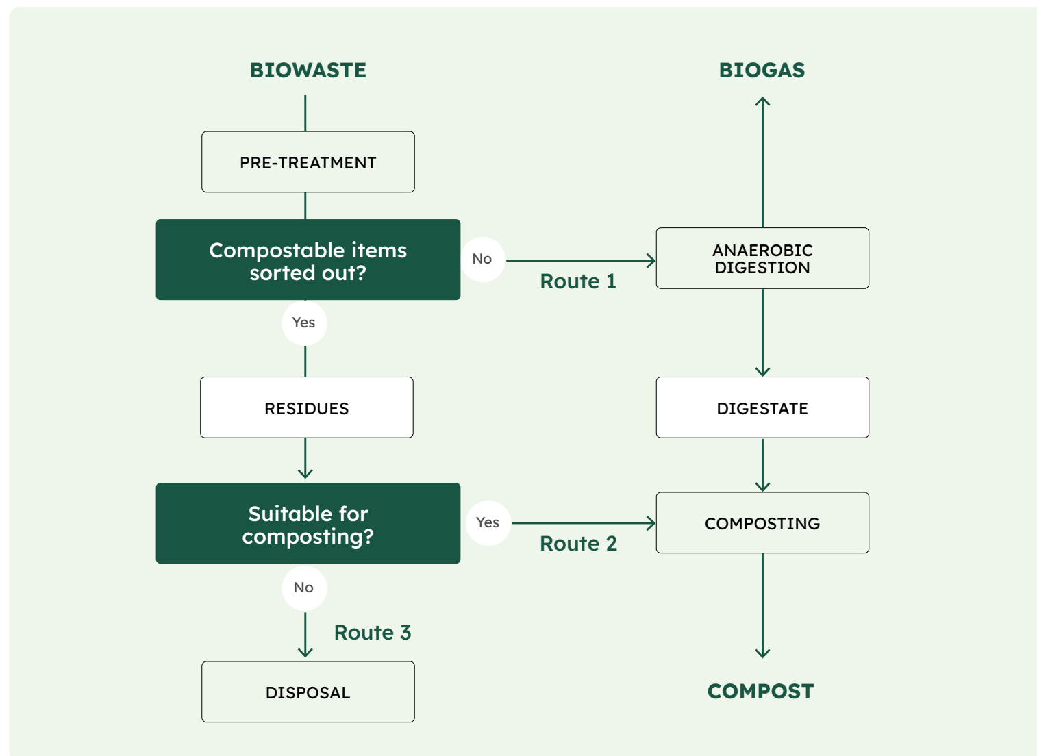
Figure 7: Routes for compostable items at anaerobic digestion facilities
