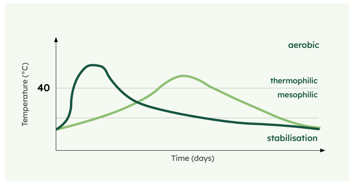
Figure 5: Temperature and microbial phases of composting
